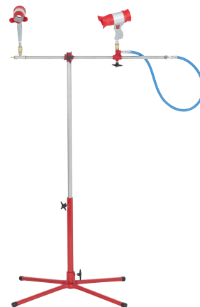
Conventional air blower paint drying system
